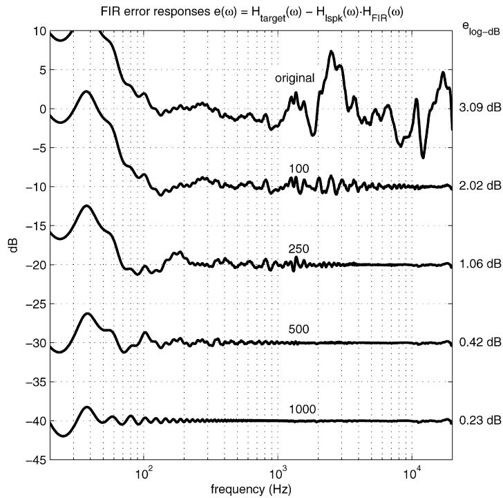
Fig. 2. Error responses (scaled 10 dB) and e_{10\text{log-dB}} value.
