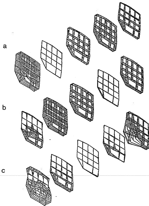
Fig. 9. Principal fields (60-100 Hz)
