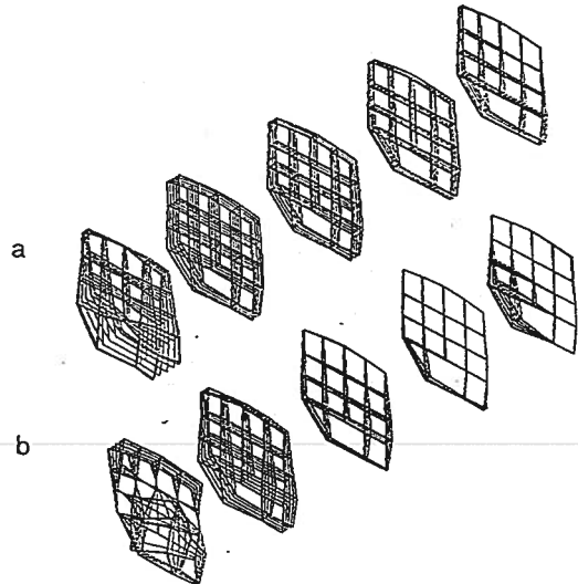
Fig. 11a,b. Principal fields 1-2 (100-140 Hz)
