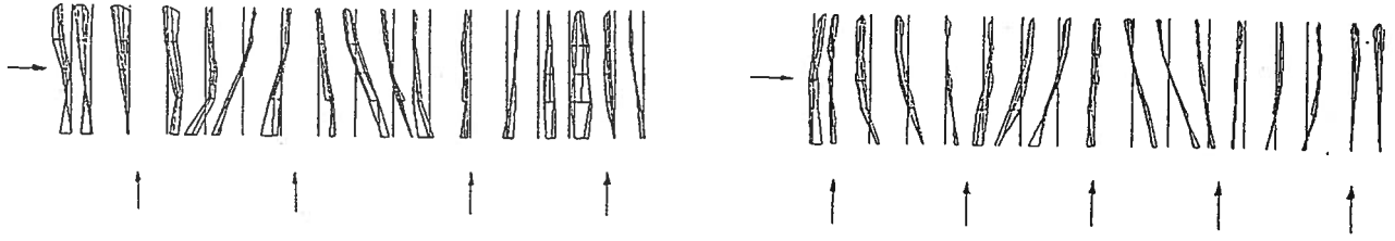
Fig. 6. 132 Hz and 166 Hz modes
