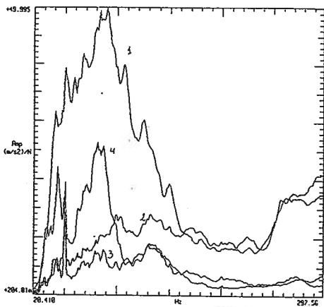
Fig. 3b. Summed FRFs (struct.)
