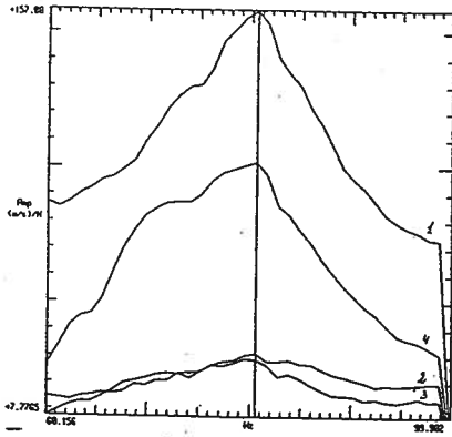
Fig. 8. Principal FRFs
