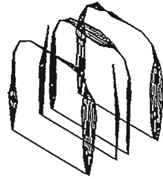
Fig. 7. 96 Hz mode shape
