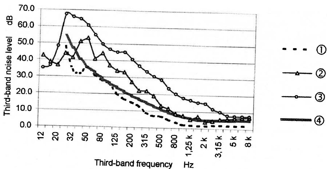
Figure 1 : Measured indoor noise in some buildings near to the planning area; (1) background noise in Studio 6, (2) reference building's cellar near to the M3-line, (3) cellar in St. Stephen's Cathedral near to the M3-line, (4) limit spectrum in radio studios.
