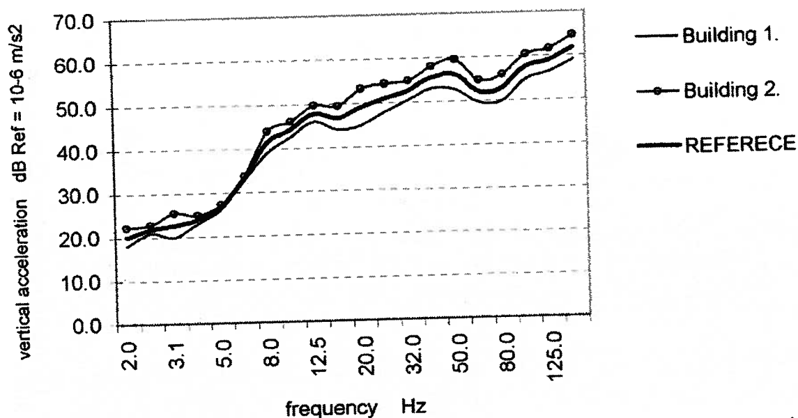
Figure 3 : The reference vibration spectrum is the arithmetic mean of two acceleration spectra, measured on two different buildings near to the existing M3-line, subtracted their dominant magnification properties, and transformed to a common reference distance.
