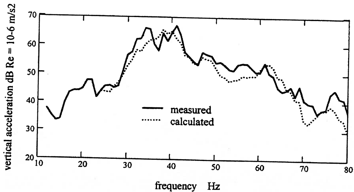
Figure 2 : Measured and calculated vertical acceleration spectra caused by a typical train passby on the ceiling of a five-storeyed reference building's cellar.
