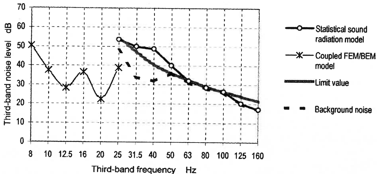
Figure 2 : Estimated indoor noise spectra from train passby in the planned tunnel.
