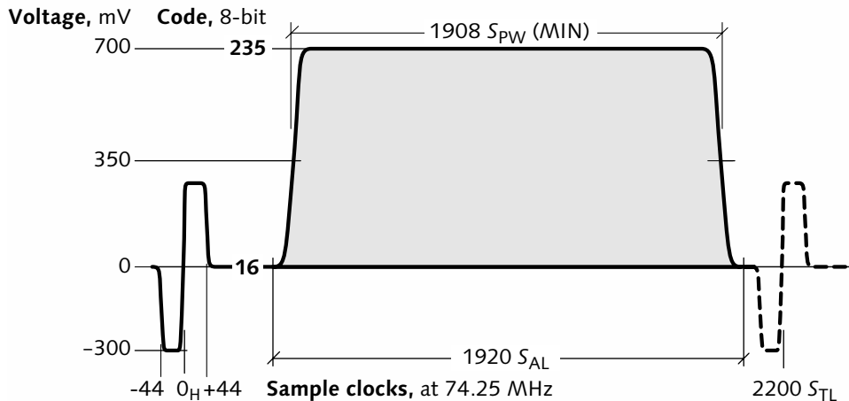
Figure 15.3 Scan-line waveform for 1080i/30 HDTV component luma. Analog trilevel sync is shown, excursions \pm 300 mV. (In digital video, sync is not coded as a signal level.) At an 8-bit interface, black is represented by code 16 and white by 235. The indicated 1920 active samples contain picture information; the remaining sample intervals of the 2200 total comprise horizontal blanking.
