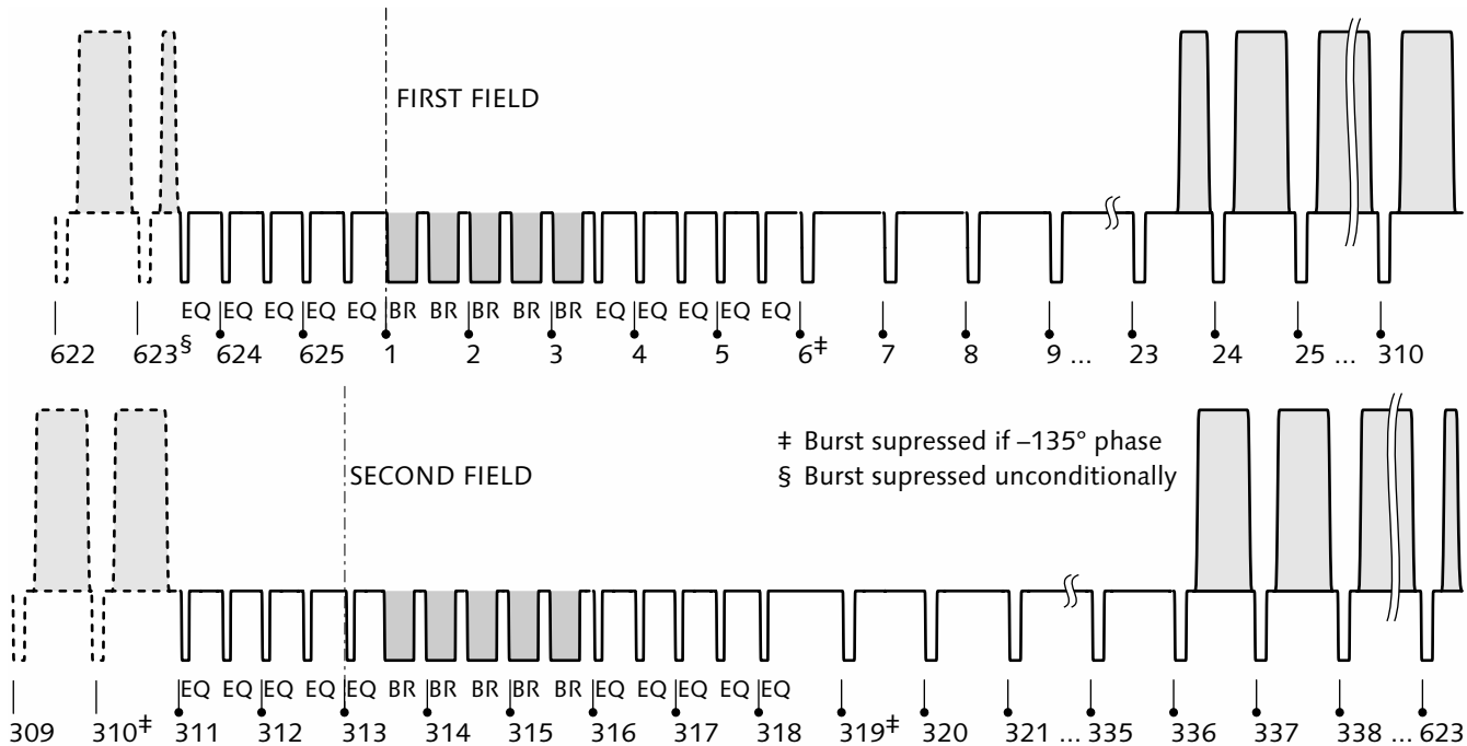
Figure 43.1 576i raster, vertical . This drawing shows waveforms of first and second fields, detailing vertical sync intervals. The first field comprises 312 lines, and the second field comprises 313 lines.
