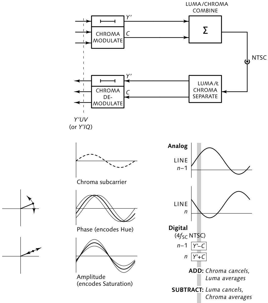
Figure 12.1 NTSC chroma modulation and frequency interleaving are applied, successively, to encode luma and a pair of color difference components into NTSC composite video. First, the two color difference signals are modulated onto a color subcarrier. If the two color differences are interpreted in polar coordinates, hue angle is encoded as subcarrier phase, and saturation is encoded as subcarrier amplitude. ( Burst , a sample of the unmodulated subcarrier, is included in the composite signal.) Then, modulated chroma is summed with luma. Frequency interleaving leads to line-by-line phase inversion of the unmodulated color subcarrier, thence to the modulated subcarrier. Summation of adjacent lines tends to cause modulated chroma to cancel, and luma to average.
