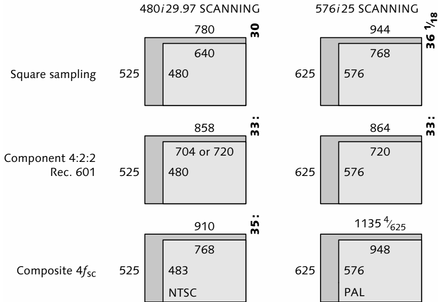
Figure 11.1 SDTV digital video rasters for 4:3 aspect ratio. 480 i 29.97 scanning is at the left, 576 i 25 at the right. The top row shows square sampling ("square pixels"). The middle row shows sampling at the Rec. 601 standard sampling frequency of 13.5 MHz. The bottom row shows sampling at four times the color subcarrier frequency ( 4f_{SC} ). Above each diagram is its count of samples per total line ( S_{TL} ); ratios among S_{TL} values are written vertically in bold numerals.
