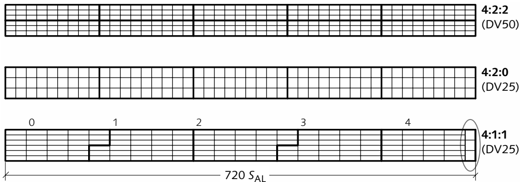
Figure 39.1 DV superblocks are shown for three chroma subsampling schemes – 4:2:2 (top), 4:2:0 (middle), and 4:1:1 (bottom). Thin lines enclose macroblocks . Each macroblock contains an 8×8 block of C_B , an 8×8 block of C_R , and two or more 8×8 blocks of luma. Thick lines enclose superblocks ; each superblock comprises 27 macroblocks. A 4:1:1 macroblock is about four times wider than it is tall.
